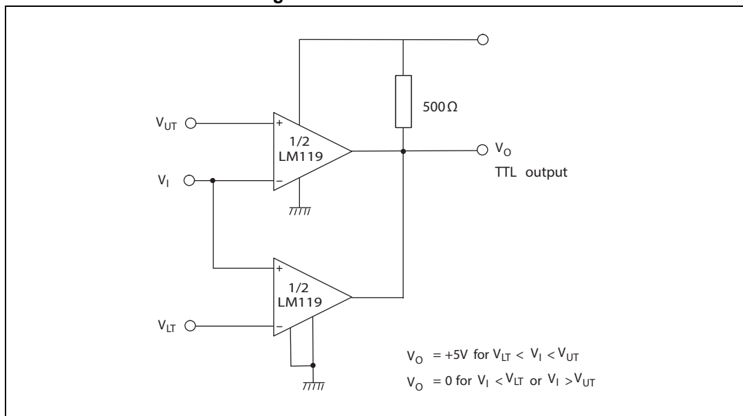
Figure 19. Window detector
