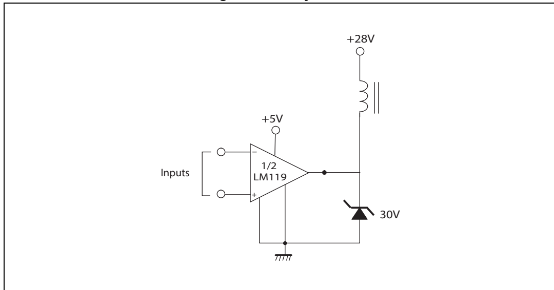
Figure 18. Relay driver
