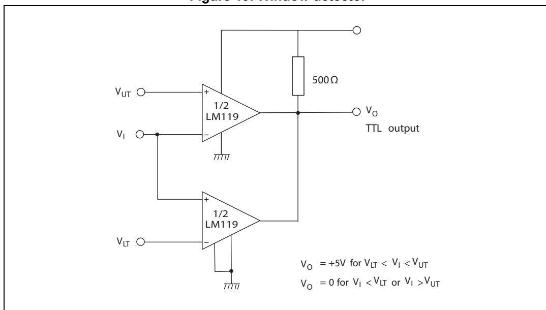
Figure 19. Window detector
