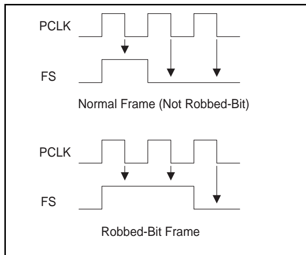
Figure 25 - Robbed-Bit Frame
