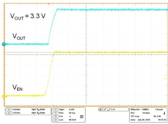
Figure 22: Enable transient
