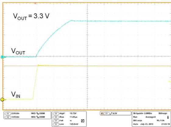
Figure 21: Start-up transient
