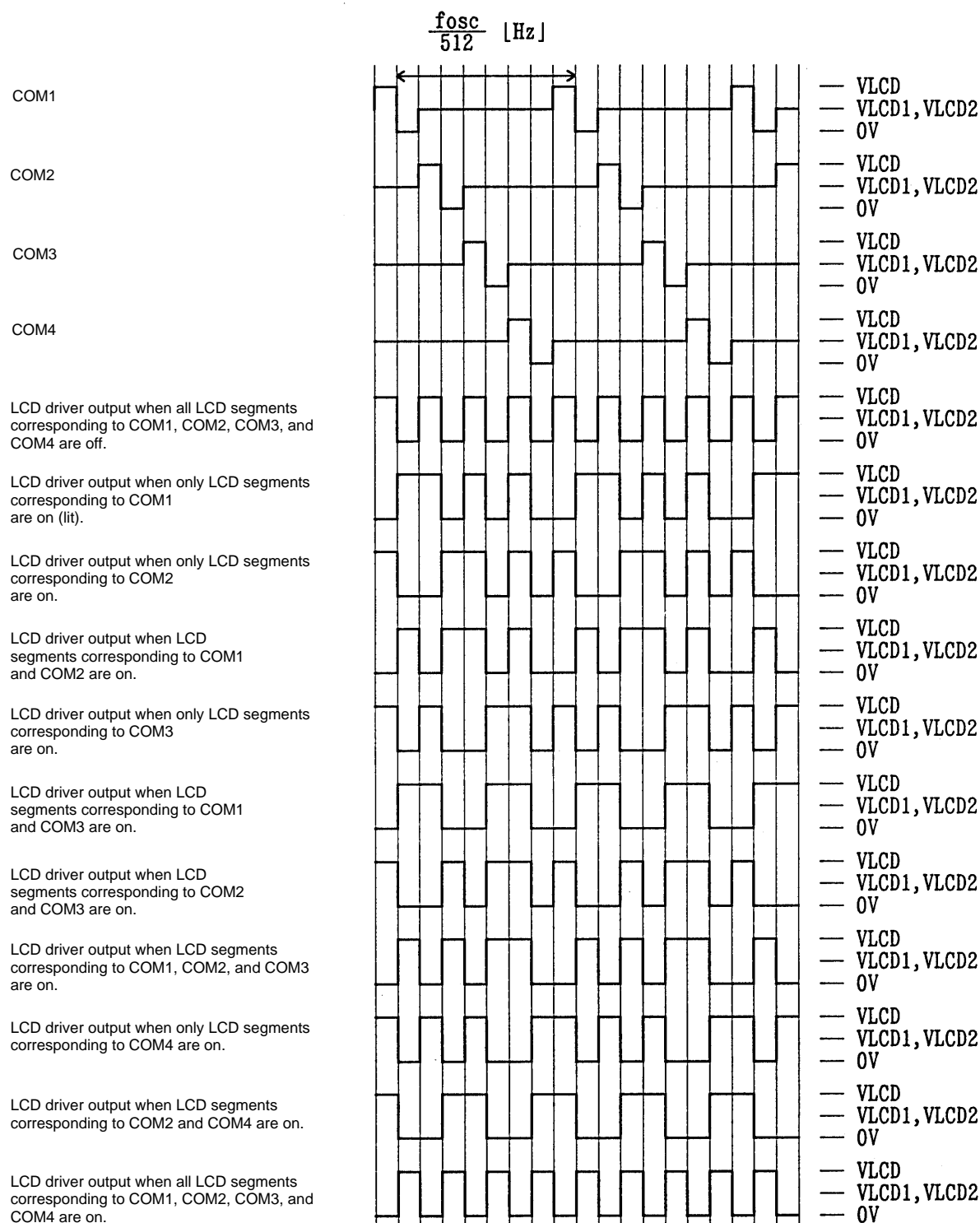
1/4-Duty 1/2-Bias Waveforms
