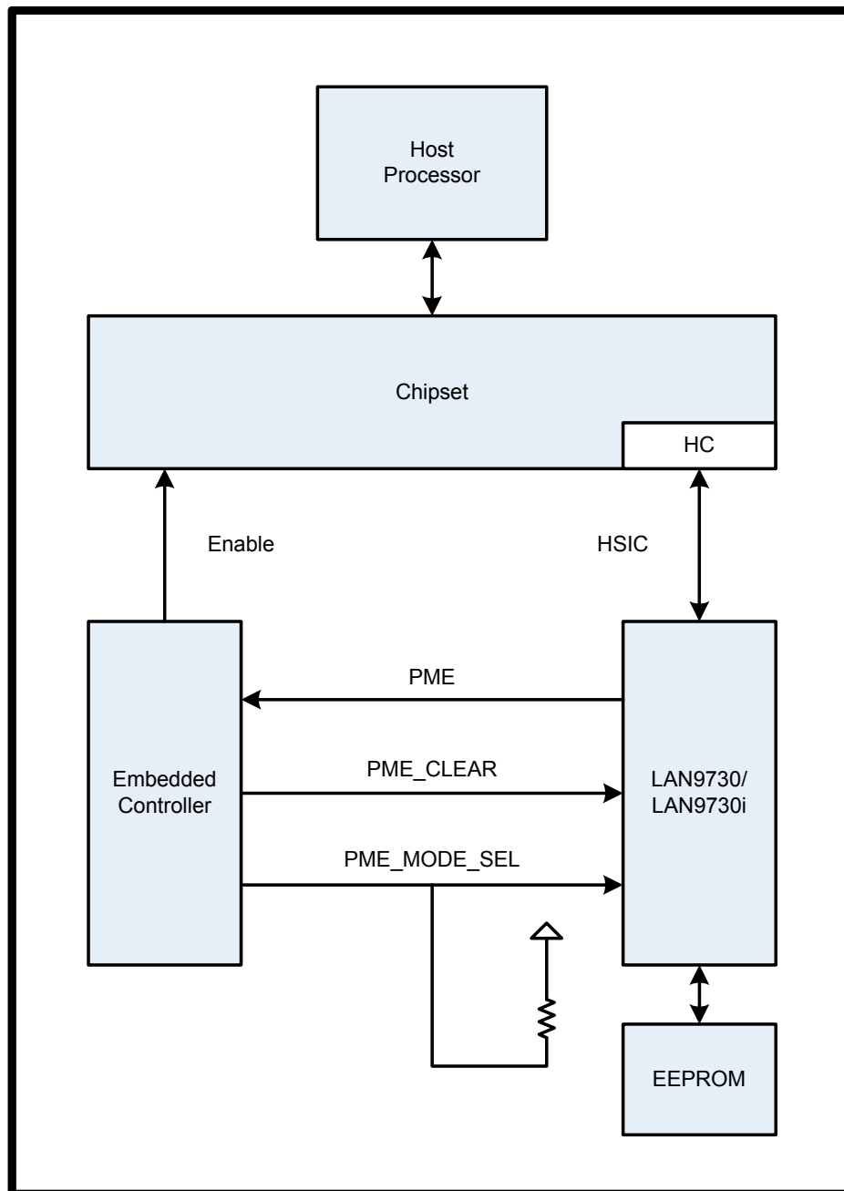
Figure 5.1 Typical Application
