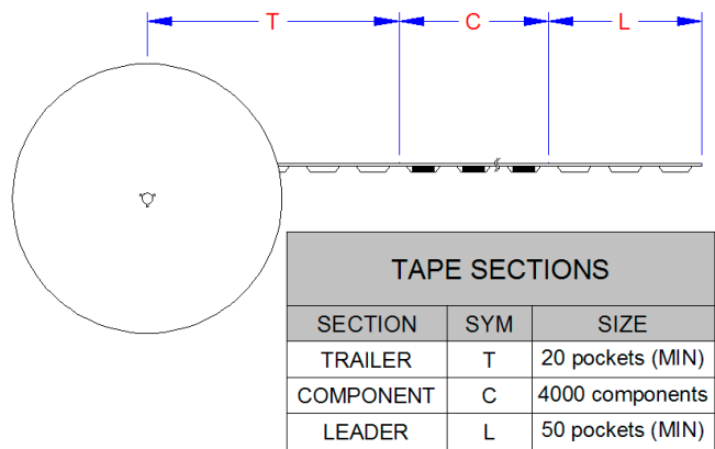
Figure 6.5 Tape Length and Part Quantity
