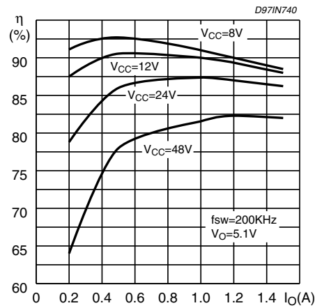
Figure 19. Efficiency vs. output current.
