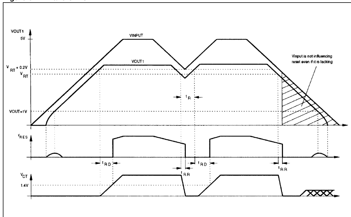
Figure 6. Waveforms
