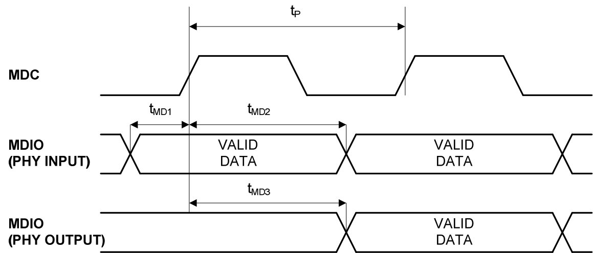
Figure 11. MDC/MDIO Timing
