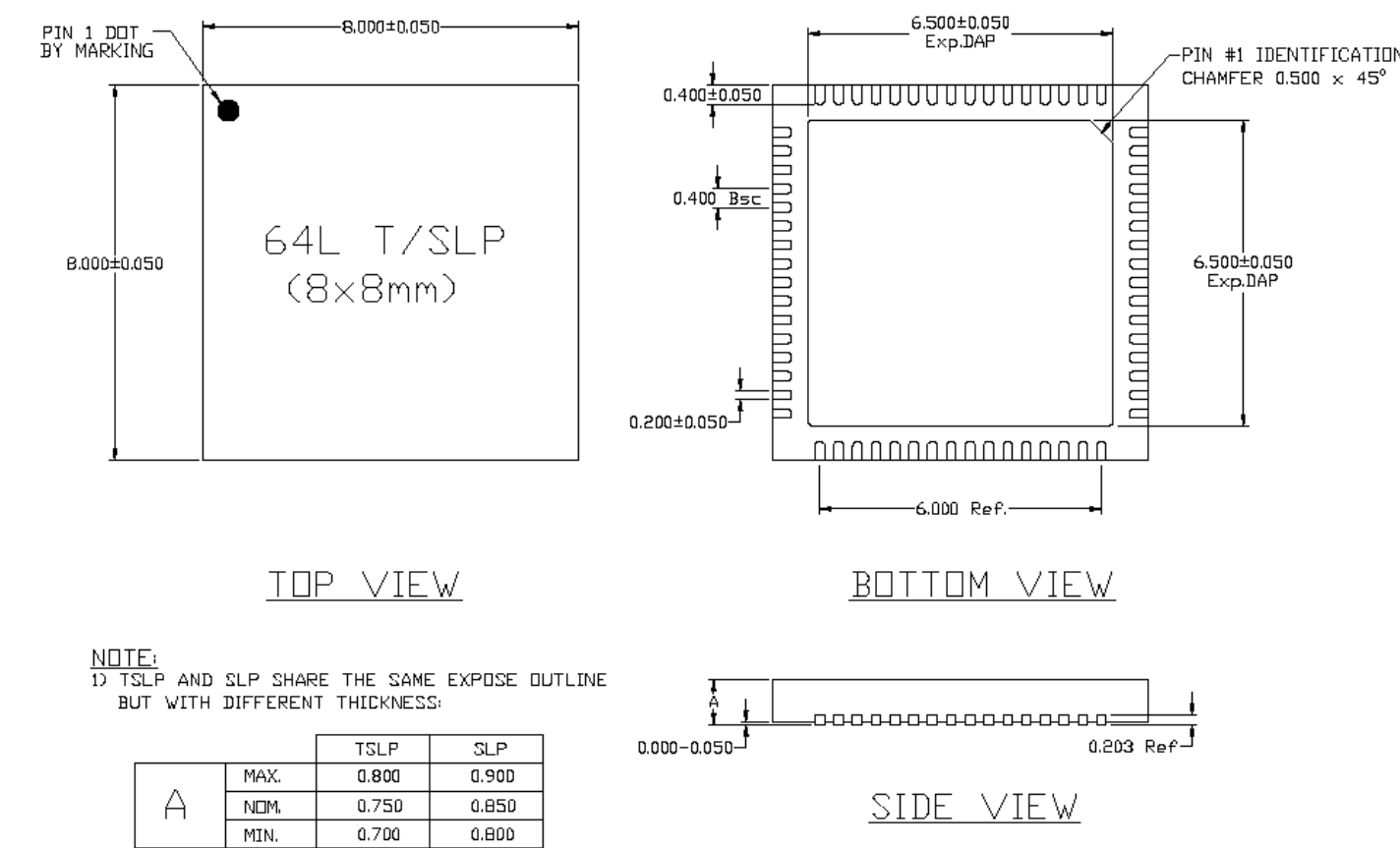
64-Pin (8mm x 8mm) QFN
