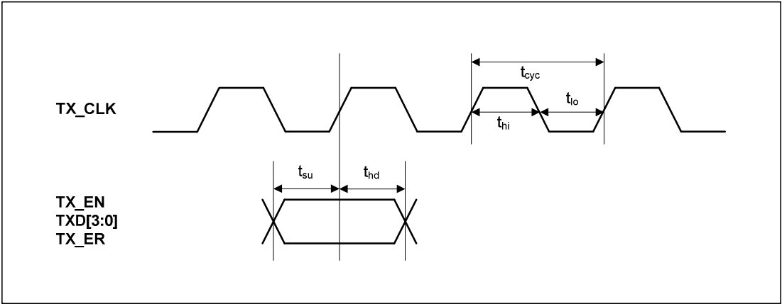
Figure 8. MII Transmit Timing – Data Input to PHY
