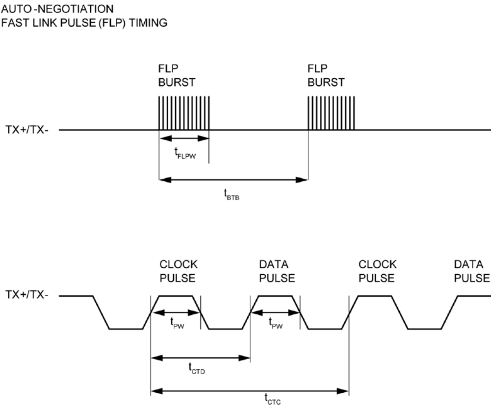
Figure 12. Auto-Negotiation Fast Link Pulse (FLP) Timing
