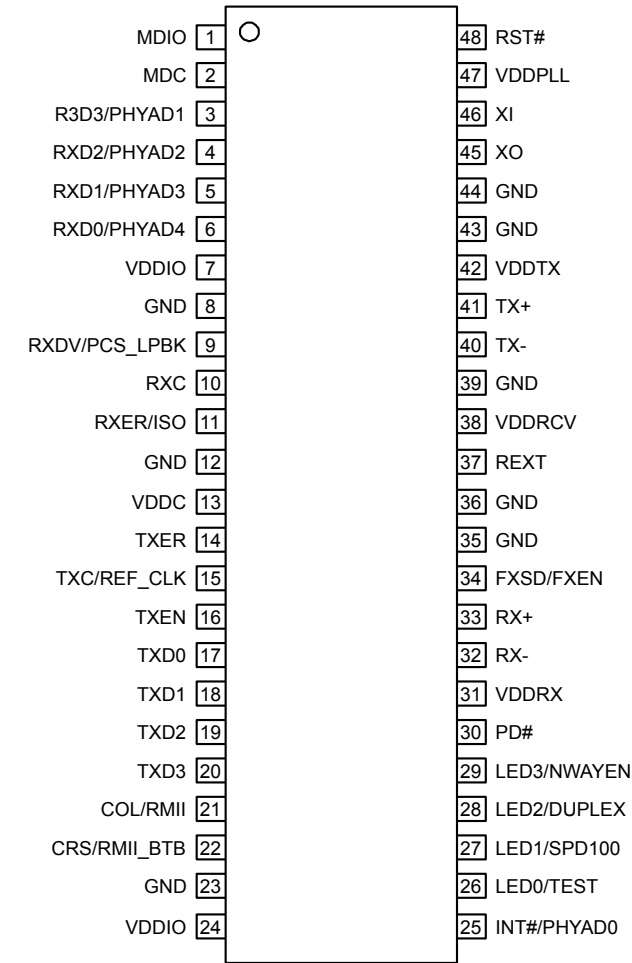
48-Pin SSOP (SM)
