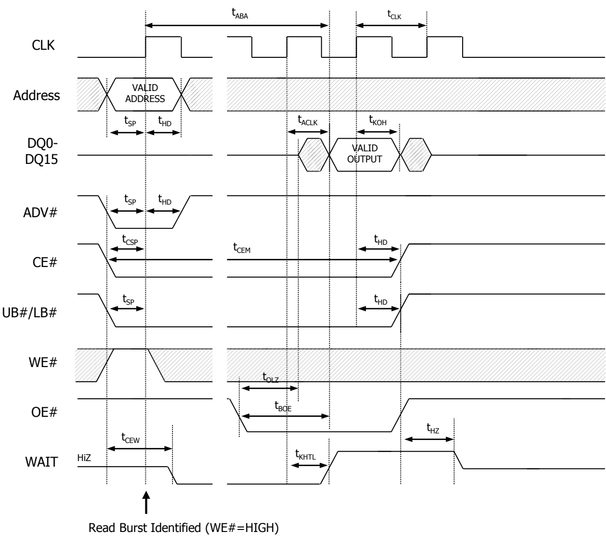
Figure 24: Single Access Burst READ Operation – Variable Latency without refresh collision
