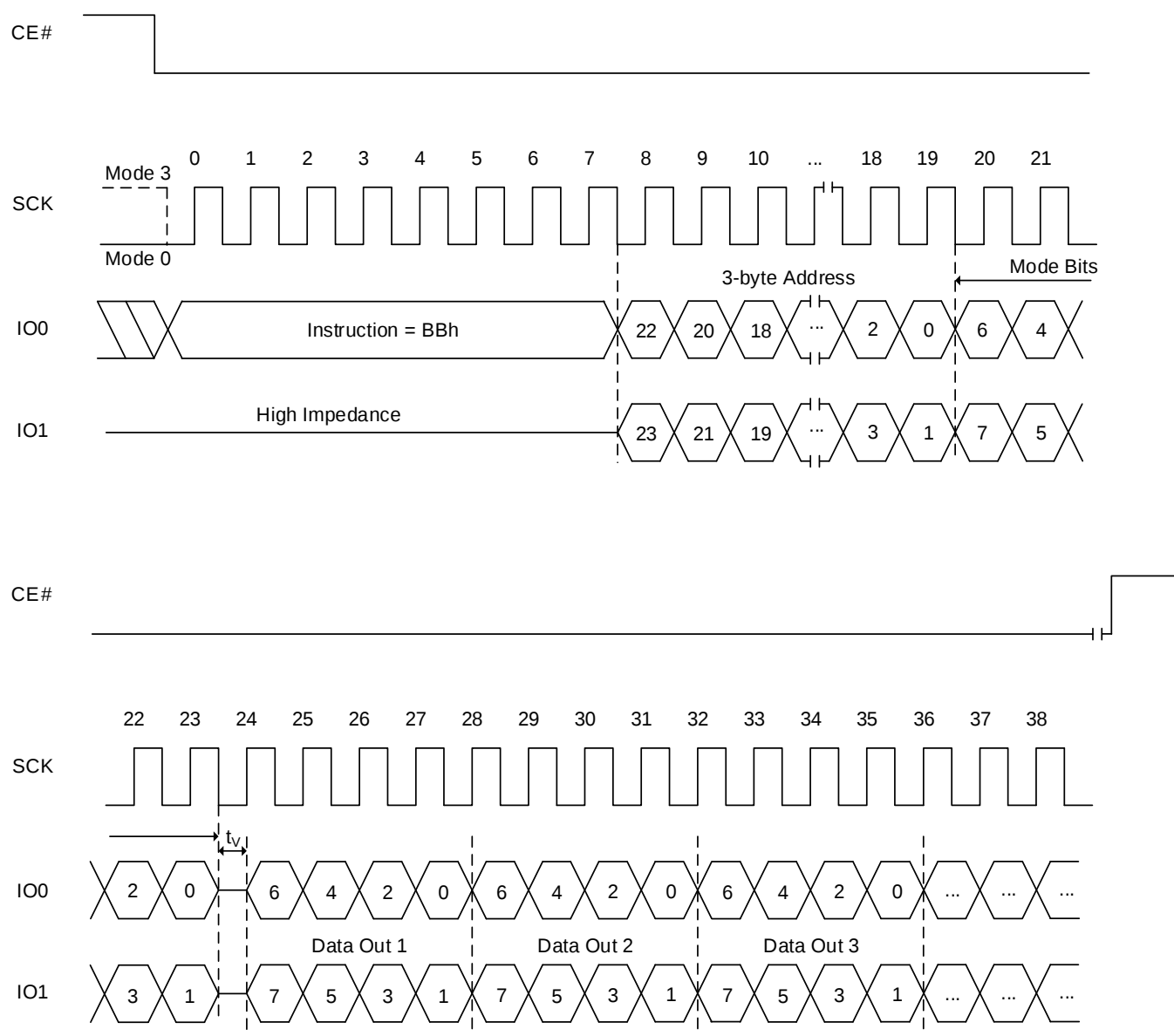
Figure 8.3 Fast Read Dual I/O Sequence (with command decode cycles)
