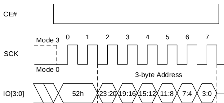
Figure 8.37 Block Erase (32K) Sequence In QPI Mode (52h [EXTADD=0], 3-byte address)
