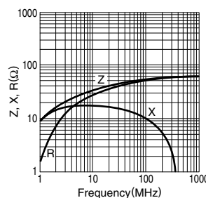
HF70ACC322513
