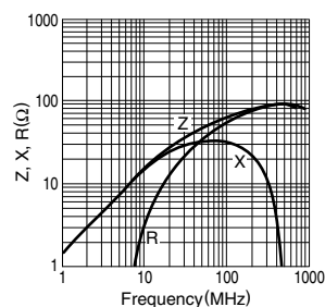
HF50ACC322513
