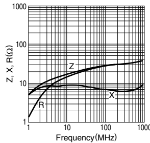
HF70ACC321611
