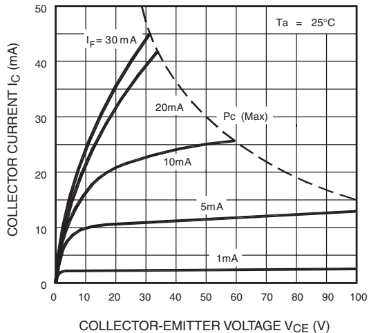
Fig. 5 Collector Current vs. Collector-Emitter Voltage (H11AA814)
