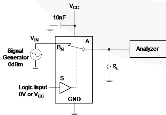
Figure 16. Bandwidth
