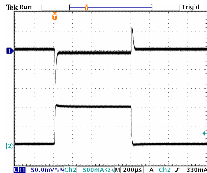
Load Transient: V_{IN} = 5.0V , V_{OUT} = 1.2V
