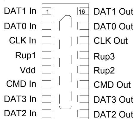
Figure 1 - Pin Identification and Configuration (Top Side View)
