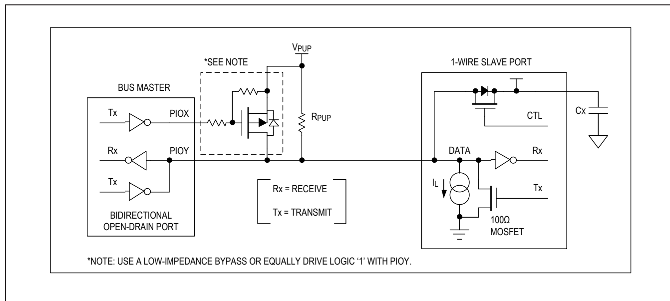
Figure 3. Hardware Configuration
