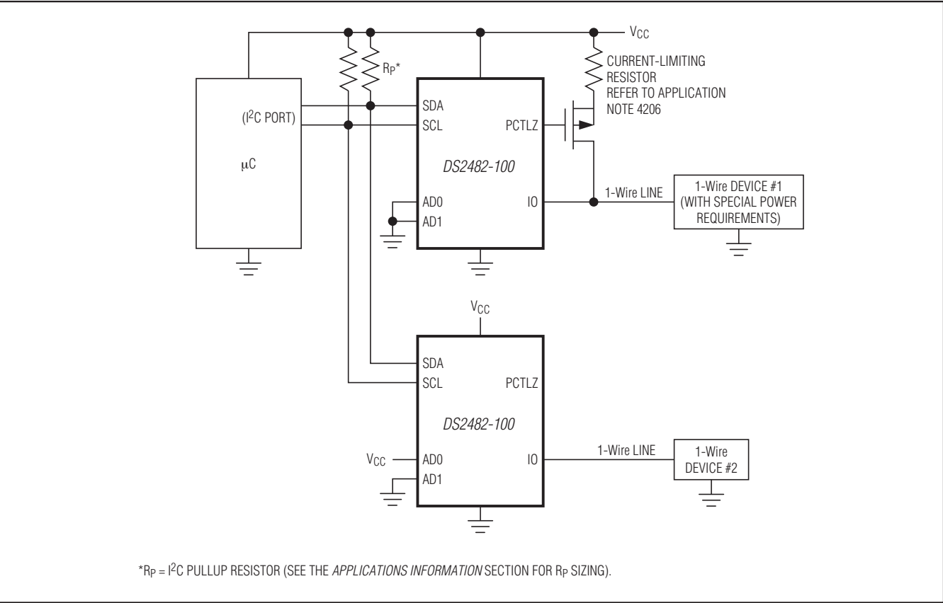
Figure 10. Application Schematic
