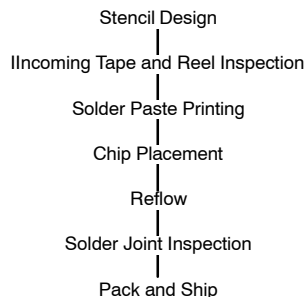
FIGURE 5. SMT Assembly Process Flow
