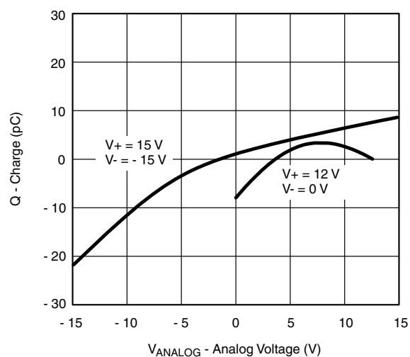
Q_S , Q_D - Charge Injection vs. Analog Voltage
