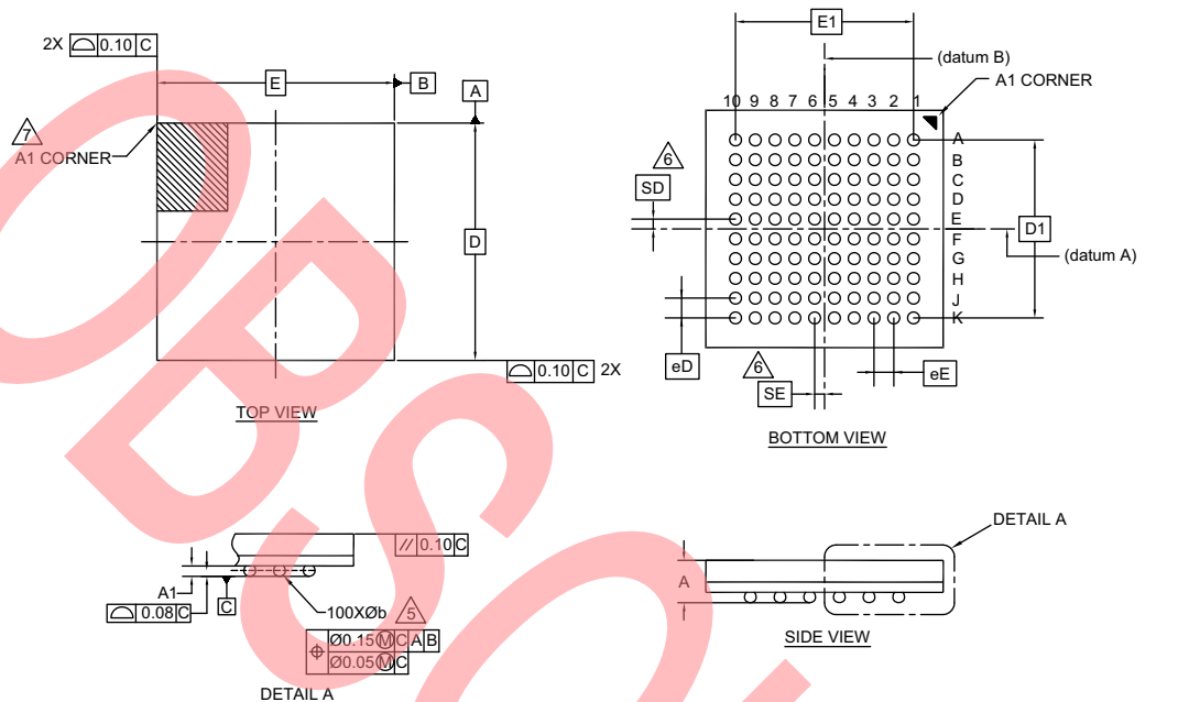
Figure 62. 100-ball VFBGA (6 × 6 × 1.0 mm) BZ100 Package Outline, 51-85209
