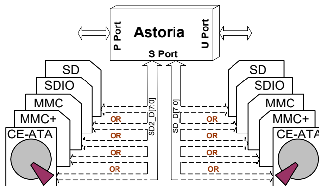
Figure 3. Dual SD/SDIO/MMC/CE-ATA Interface Mode
