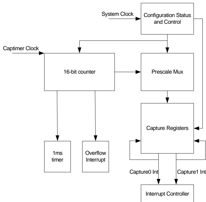
Figure 10. Timer Capture Block Diagram
