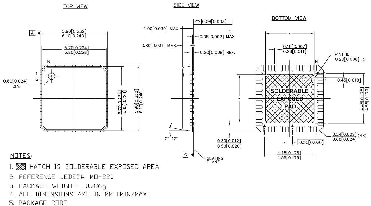
Figure 32. 40-pin QFN (6 × 6 × 1.0 mm) LF40A/LY40A (3.50 × 3.50 mm) E-Pad (Punch) Package Outline, 001-12917 [15]
