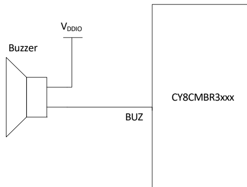
Figure 8. Buzzer Connection [9]
