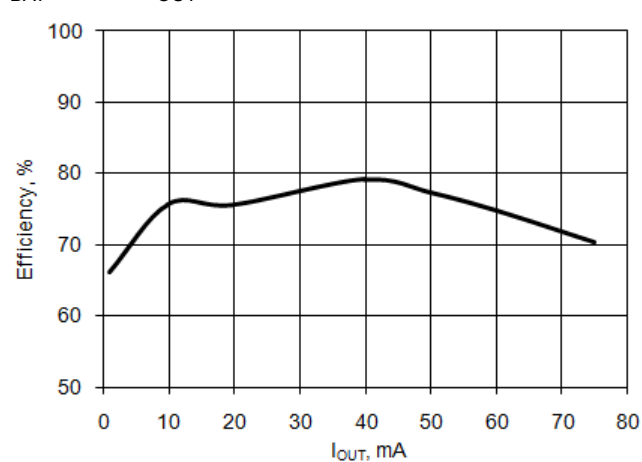
Figure 11-11. Efficiency vs I_{\text{OUT}}
