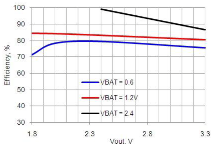
Figure 11-10. Efficiency vs V_{\text{OUT}}
