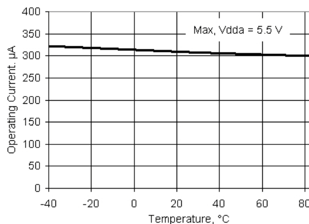
Figure 11-56. VDAC Operating Current vs Temperature, 1 V Mode, High speed mode
