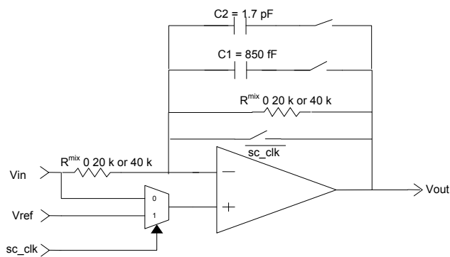
Figure 8-13. Mixer Configuration
