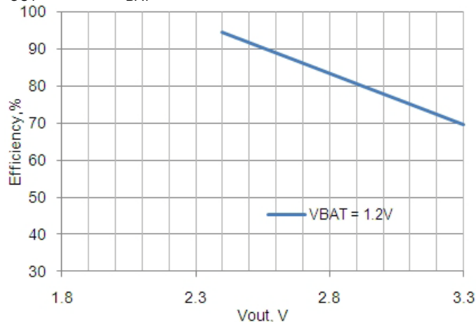
Figure 11-10. Efficiency vs V_{\text{OUT}}
