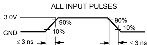
Figure 4. AC Test Loads and Waveforms [9, 10]
