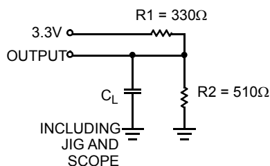
Figure 4. AC Test Loads and Waveforms [9, 10]
