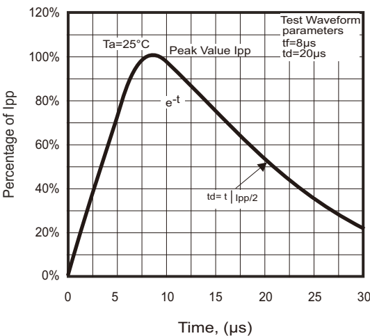
Fig.3 - 8/20 \mu\text{s} Peak Pulse Current Waveform Acc. IEC 61000-4-5
