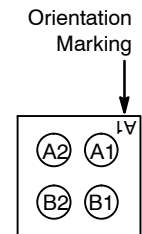
CM1230-02/J2 4-bump CSP Package
