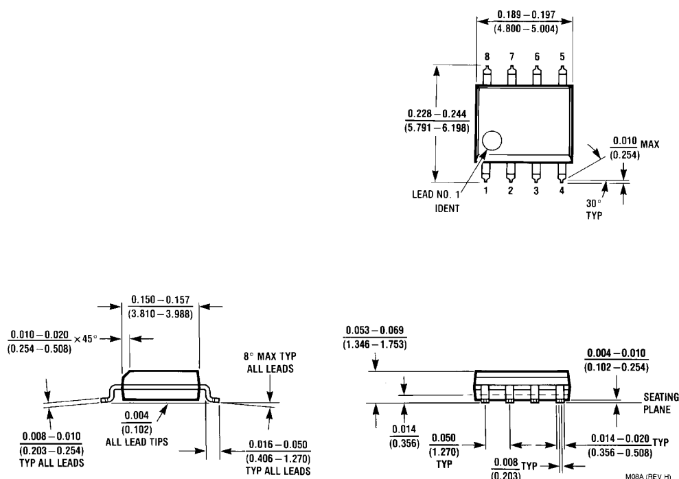
8-Lead Small Outline Integrated Circuit (SOIC), JEDEC MS-012, 0.150" Narrow Body Package Number MO8A
