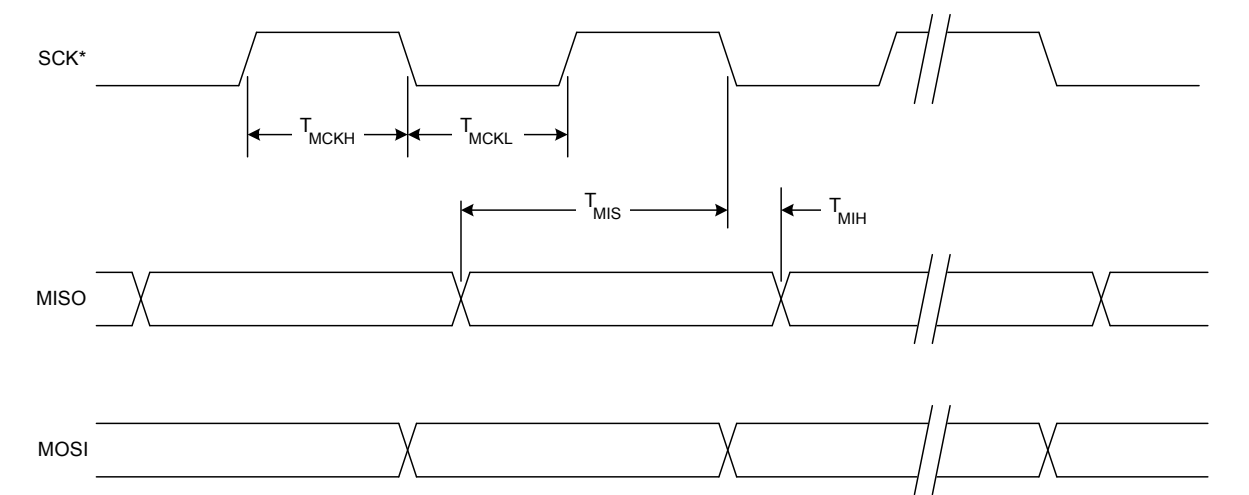
Figure 30.8. SPI Master Timing (CKPHA = 0)
