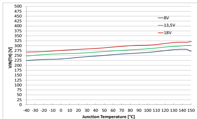
Figure 51 Input Voltage Hysteresis V_{IN(HYS)} = f(T_J; V_S)
