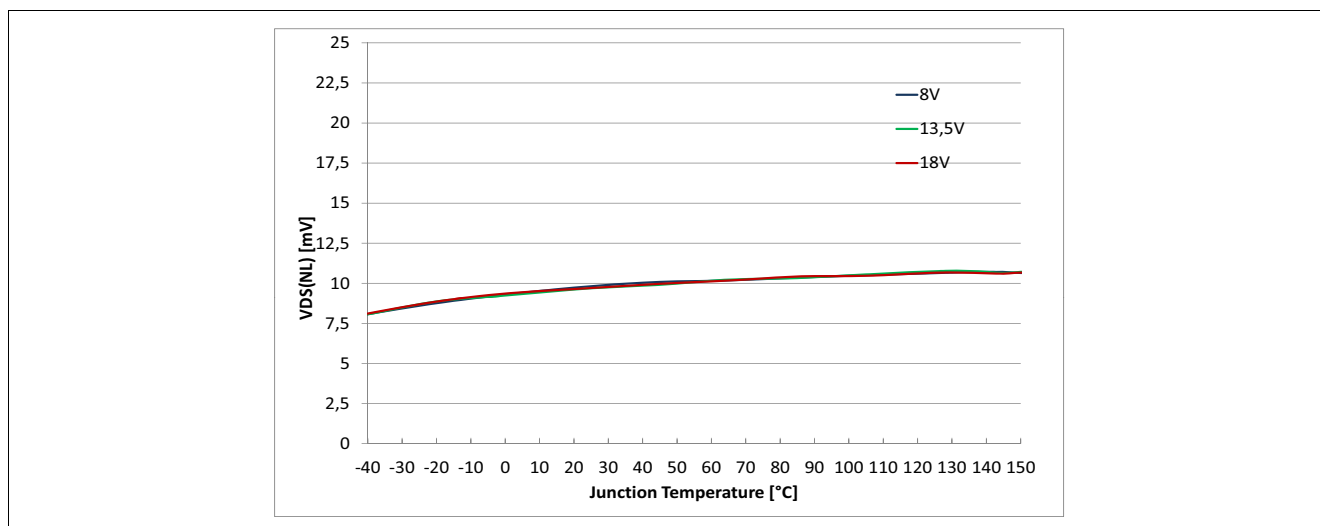
Figure 34 Output Voltage Drop Limitation at Low Load Current V_{DS(NL)} = f(T_J; V_S)
