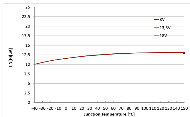
Figure 52 Input Current High Level I_{IN(H)} = f(T_J; V_S)
