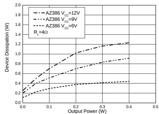
Figure 9. Device Dissipation vs. Output Power ( 4\Omega Load)
