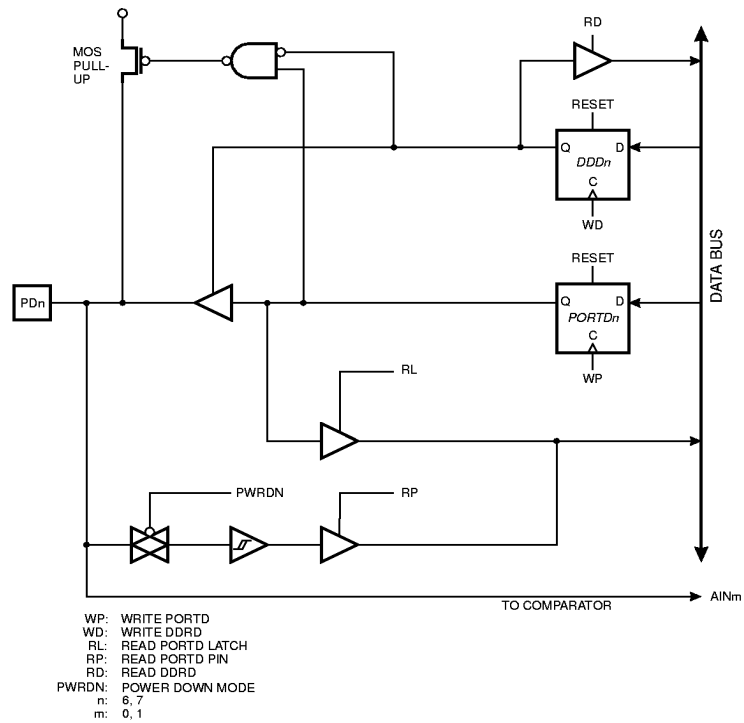
Figure 61. Port D Schematic Diagram (Pins PD6 and PD7)
