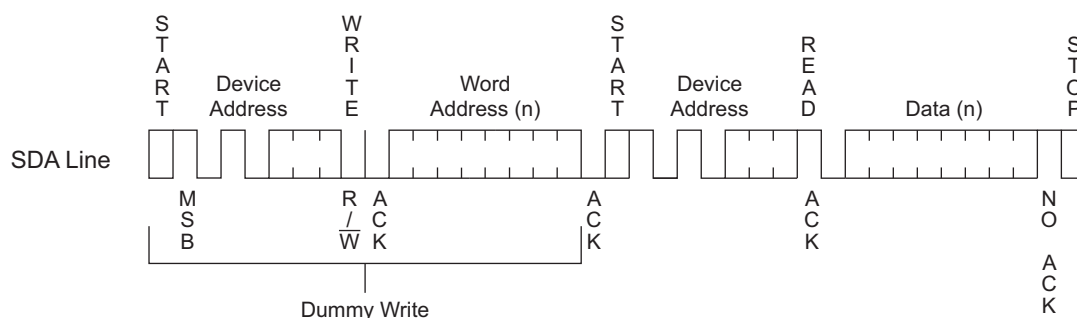
Figure 9-2. Random Read
