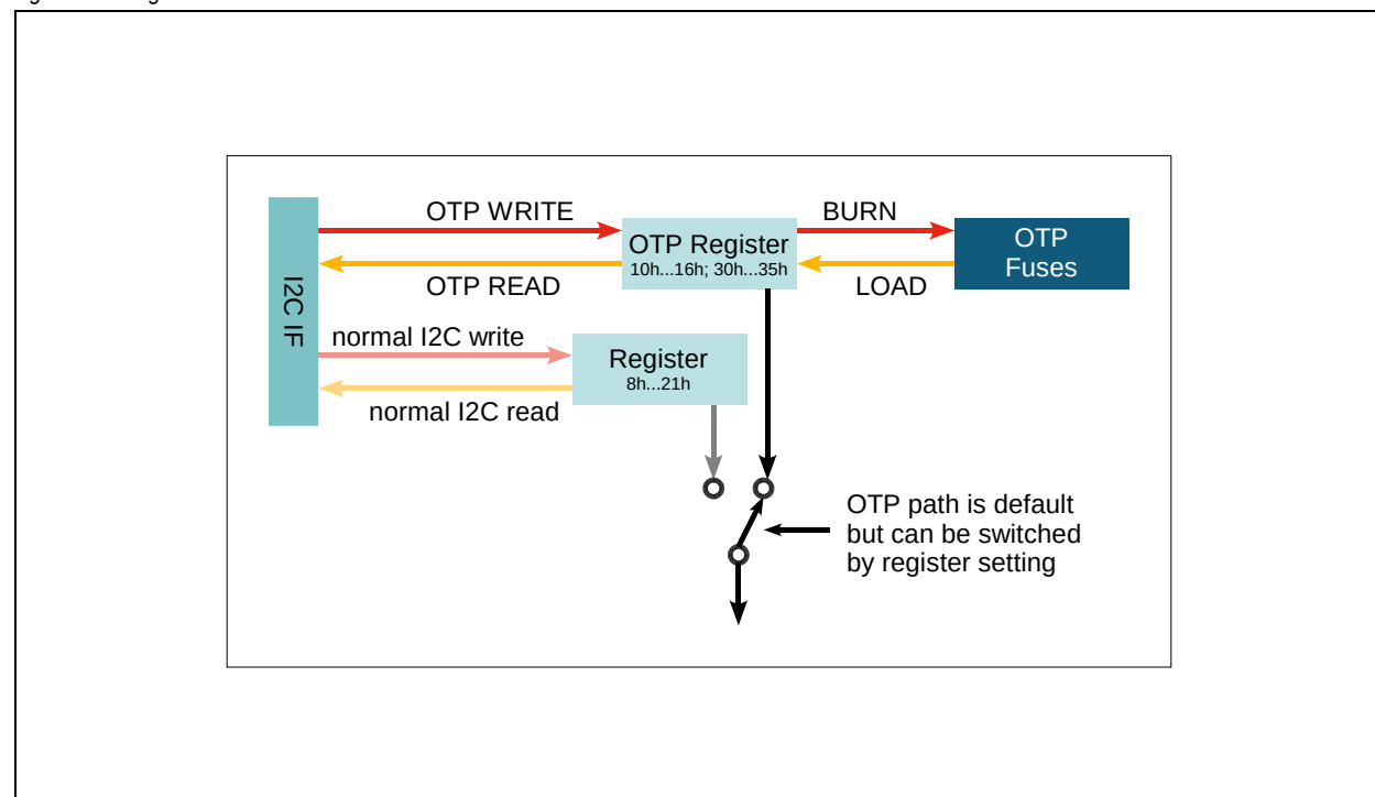
Figure 19. Register Access
