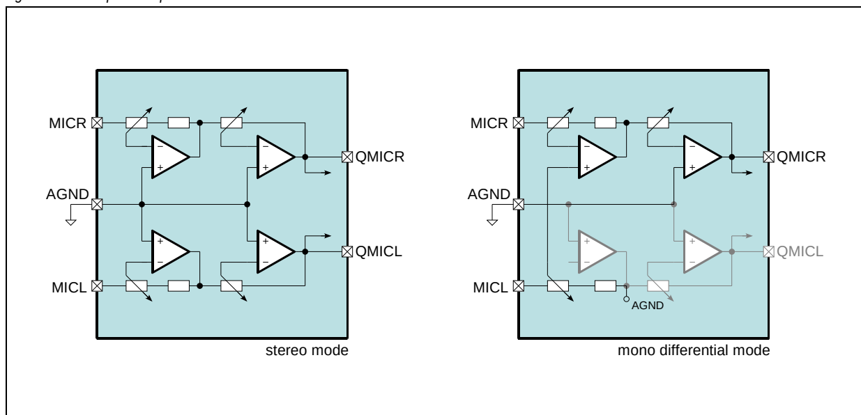
Figure 13. Microphone Input
