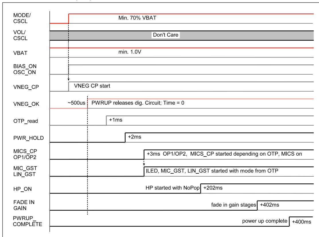
Figure 17. Stand-Alone Mode Start-Up Sequence
