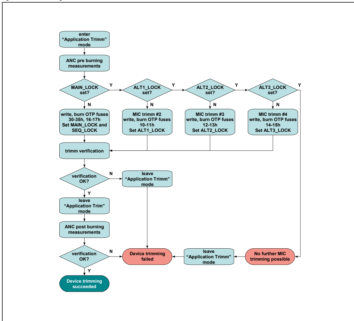
Figure 20. OTP Burning Process
