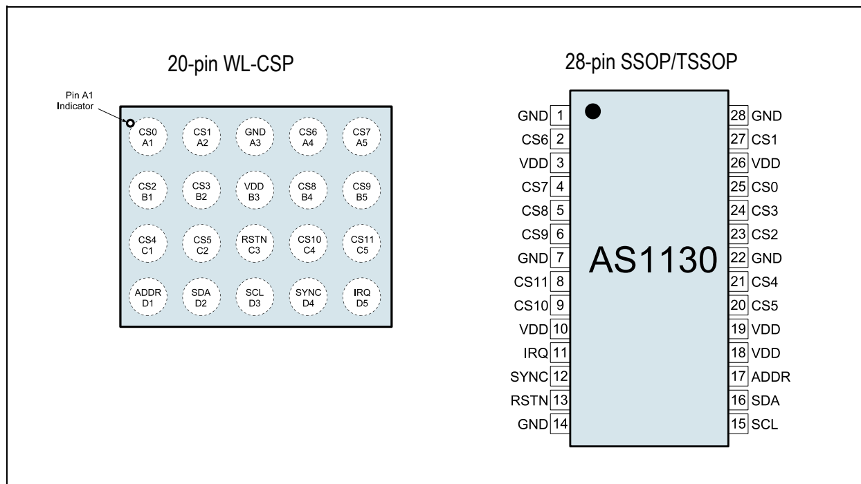
Figure 4: Pin Diagram (Top View)
