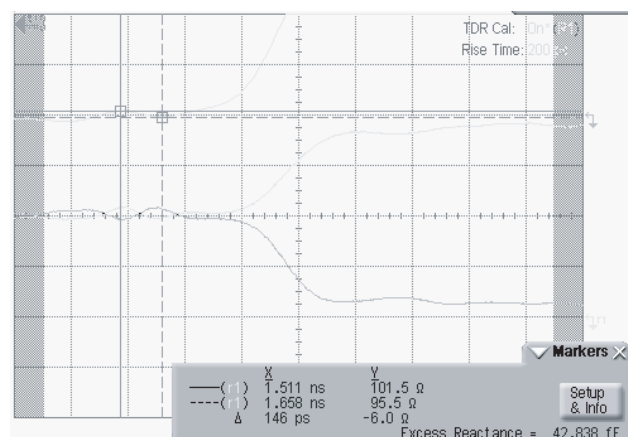
Figure 13. 160Ω Differential Impedance with AOZ8007 MSOP-10 Package on it Max. 101Ω, Min. 95Ω
