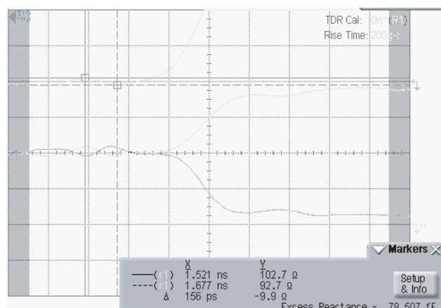
Figure 12. 140Ω Differential Impedance with AOZ8007 MSOP-10 Package on it Max. 102Ω, Min. 92Ω
