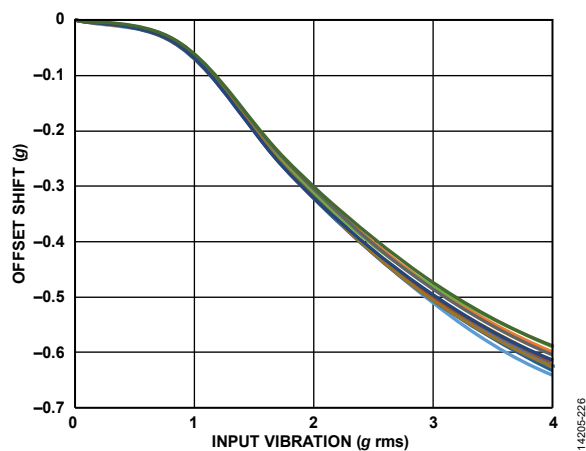
Figure 27. ADXL354 VRE, Y-Axis Offset from +1 g, ±2 g Range, Y-Axis Orientation = +1 g
