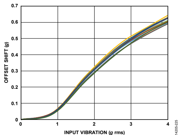
Figure 26. ADXL354 VRE, X-Axis Offset from -1 g, ±2 g Range, X-Axis Orientation = -1 g
