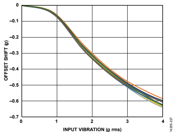
Figure 28. ADXL354 VRE, Z-Axis Offset from +1 g, ±2 g Range, Z-Axis Orientation = +1 g
