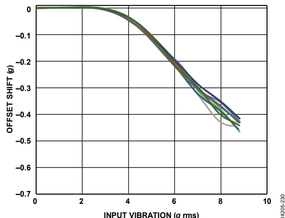
Figure 31. ADXL354 VRE, Z-Axis Offset from +1 g, ±8 g Range, Z-Axis Orientation = +1 g
