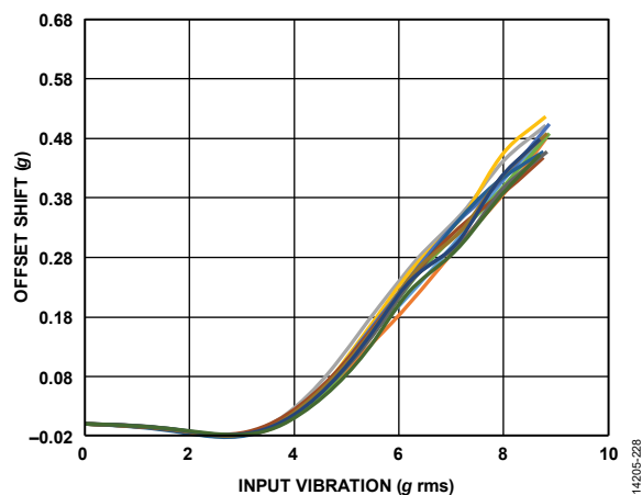
Figure 29. ADXL354 VRE, X-Axis Offset from -1 g, ±8 g Range, X-Axis Orientation = -1 g
