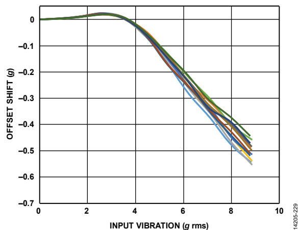
Figure 30. ADXL354 VRE, Y-Axis Offset from +1 g, ±8 g Range, Y-Axis Orientation = +1 g
