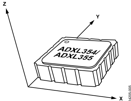
Figure 60. Axes of Acceleration Sensitivity
