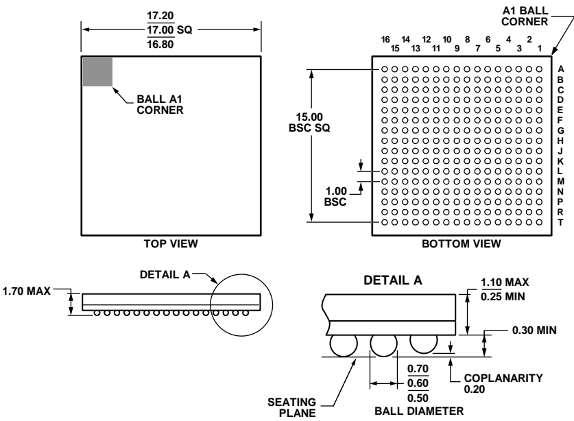
Figure 10. 256-Ball Chip Scale Package Ball Grid Array [CSP_BGA] (BC-256-3) Dimensions shown in millimeters
