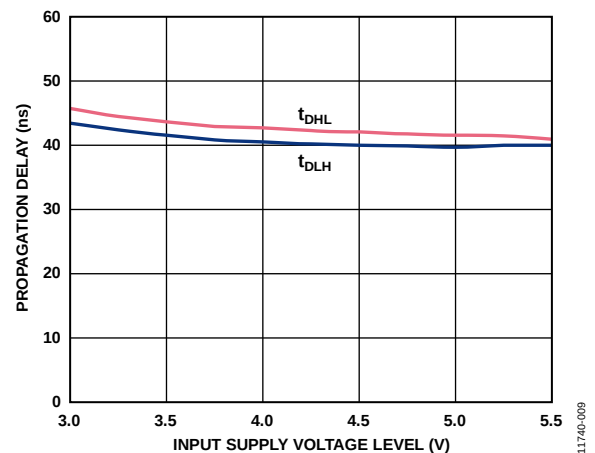
Figure 9. Typical Propagation Delay vs. Input Supply Voltage, V_{DD1}/V_{DDB} = 12 V
