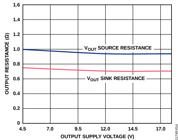
Figure 14. Typical Output Resistance vs. Output Supply Voltage
