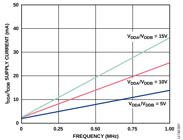
Figure 7. Typical I_{DD1}/I_{DDB} Supply Current vs. Frequency with 2 nF Load
