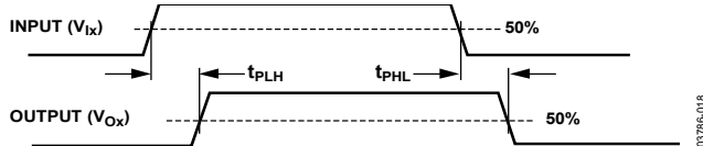
Figure 18. Propagation Delay Parameters
