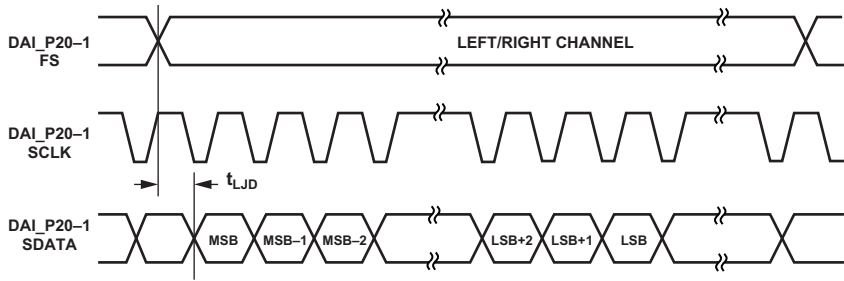
Figure 31. Left-Justified Mode
