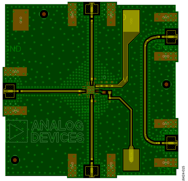
Figure 15. ADRF5132-EVALZ Evaluation Board Layout
