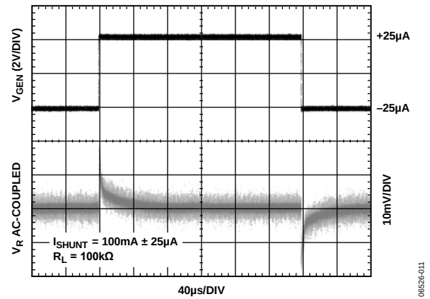
Figure 11. ADR5045 Load Transient Response
