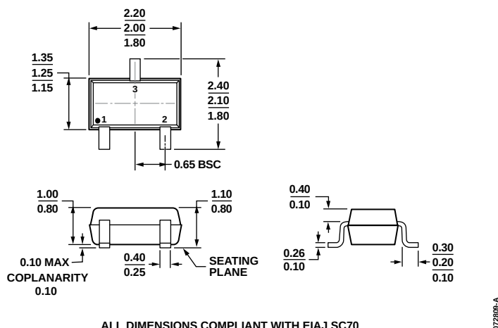
Figure 24. 3-Lead Thin Shrink Small Outline Transistor Package [KS-SC-70] (KS-3)
