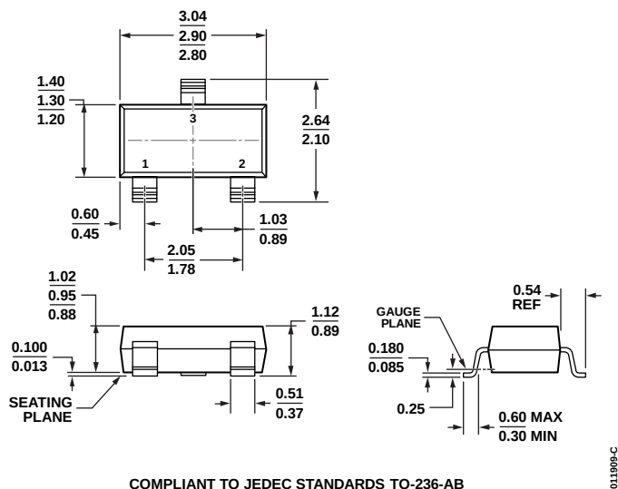
Figure 25. 3-Lead Small Outline Transistor Package [RT-SOT-23-3] (RT-3)
