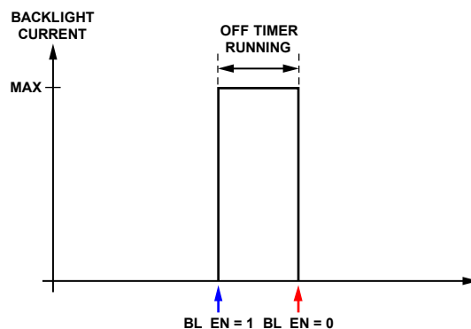
Figure 35. Off Timer
