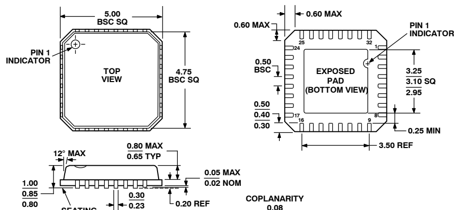
Figure 18. 32-Lead Lead Frame Chip Scale Package [LFCSP_VQ] 5 mm x 5 mm Body, Very Thin Quad (CP-32-2)
