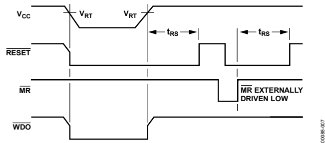
Figure 13. \overline{RESET} , \overline{MR} , and \overline{WDO} Timing
